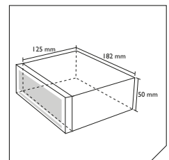
Depth: 125mm
